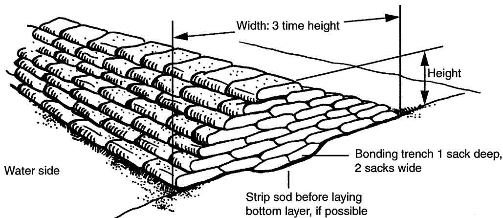
Stacking sandbags with a base width three times the height
